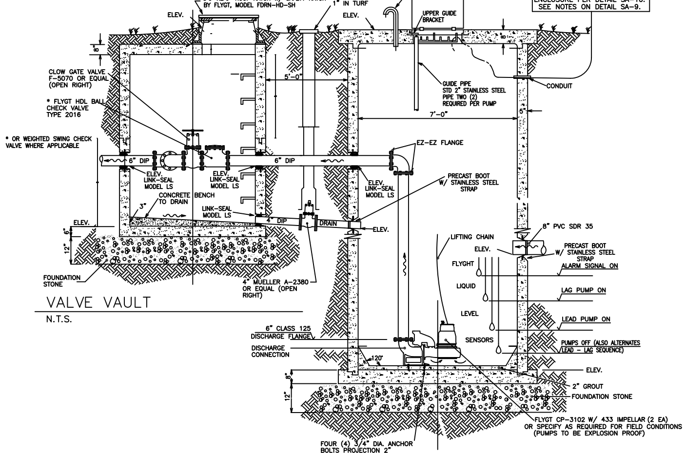
FLYGT PUMP STATION N.T.S.
