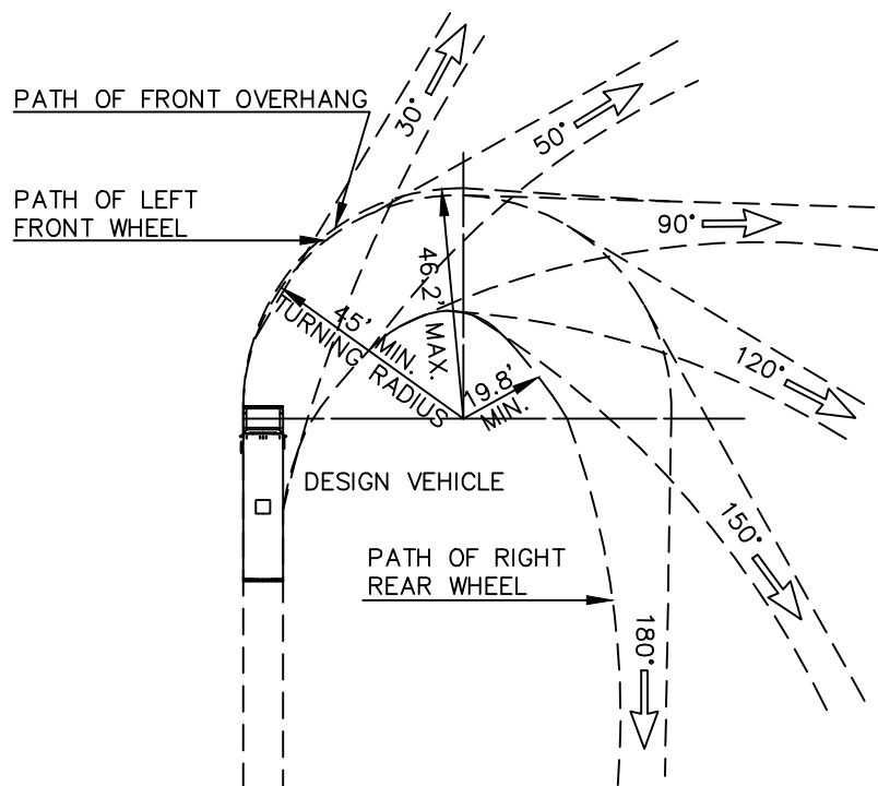
MINIMUM TURNING PATH FOR WB-50 DESIGN VEHICLE (TRACTOR TRAILER)
