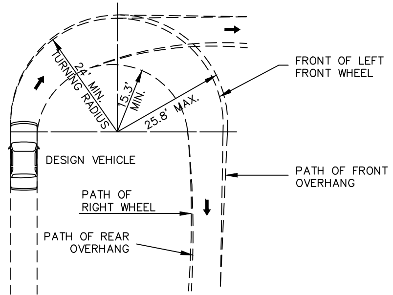
MINIMUM TURNING PATH FOR P DESIGN VEHICLE (PASSENGER VEHICLE)
